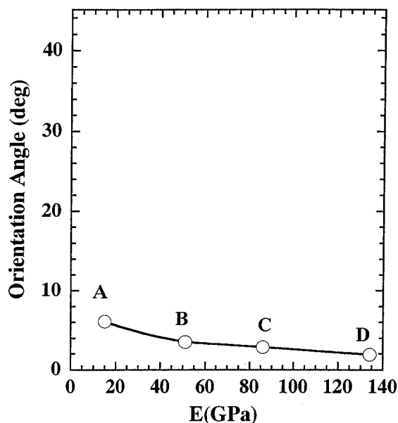
Figure 6 Orientation angles and tensile modulus of DF(A-D).
