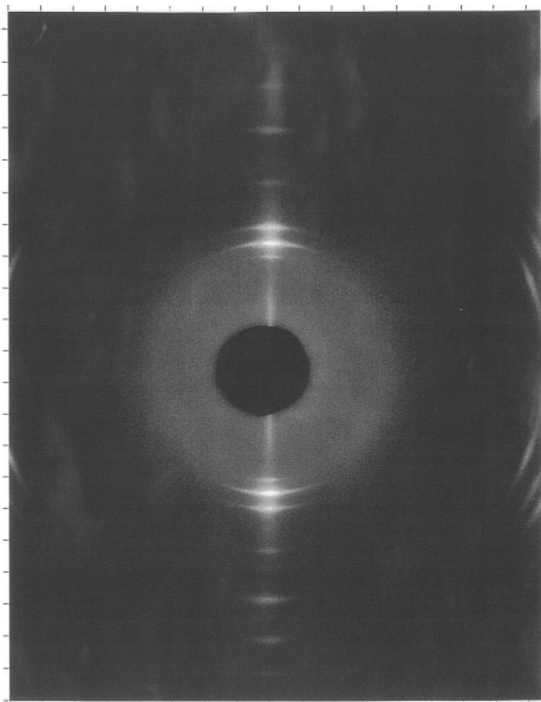
Figure 5 X-ray diffraction photograph of DF(A).
